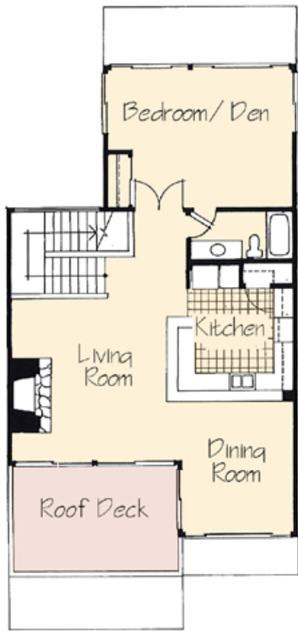
Upper Level
