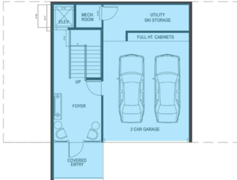
Ground Level Floorplan
